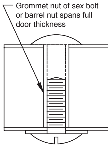
Figure 6 – Proper thru-bolting
