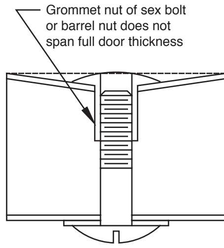
Figure 7 – Improper thru-bolting
